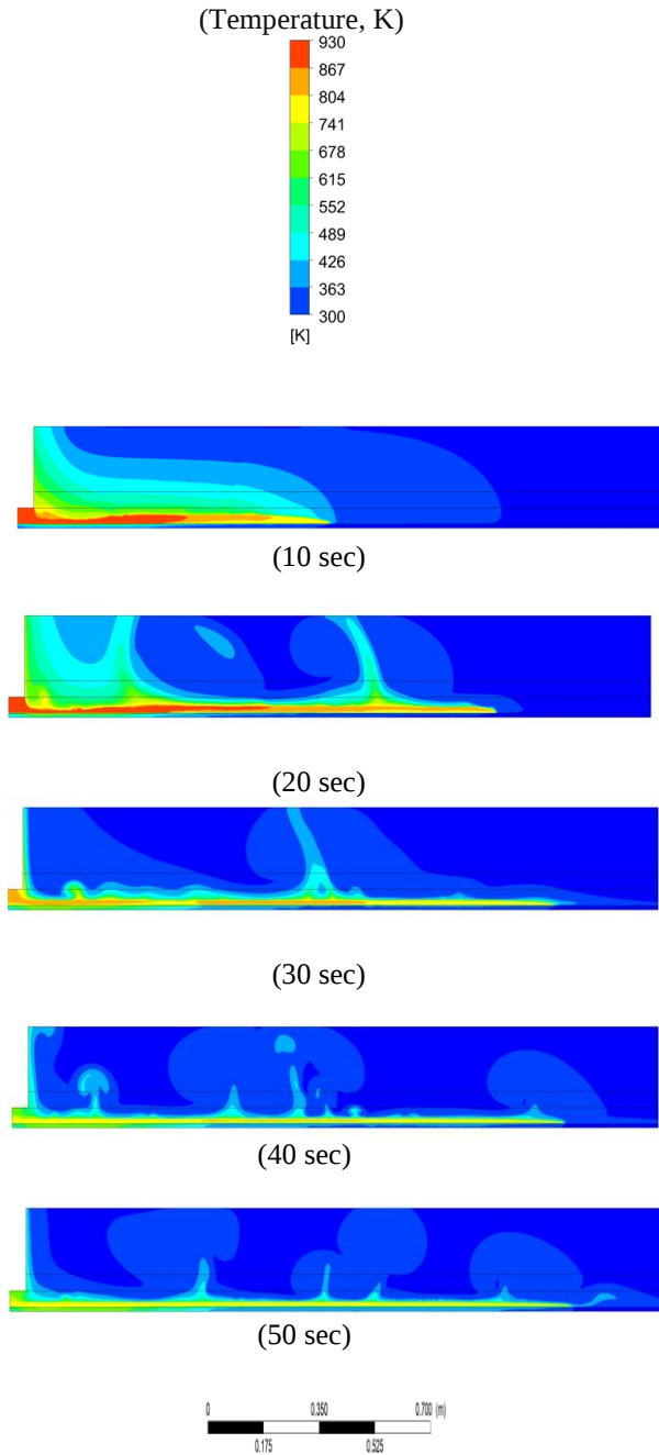
Fig. 4 ANSYS-Fluent results on temperature distribution of the spill molten salt with time increase (KCl-NaCl- \text{UCl}_3 ).
