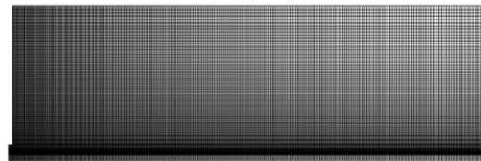
Fig. 2 ANSYS-Fluent mesh for spreading and cooling analysis of the spill molten salt.
