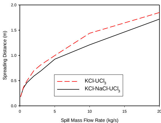
Fig. 7 ANSYS-Fluent results on spreading distance of the spill molten salt for 20 sec as function of spill mass flow rate at 120 sec.
