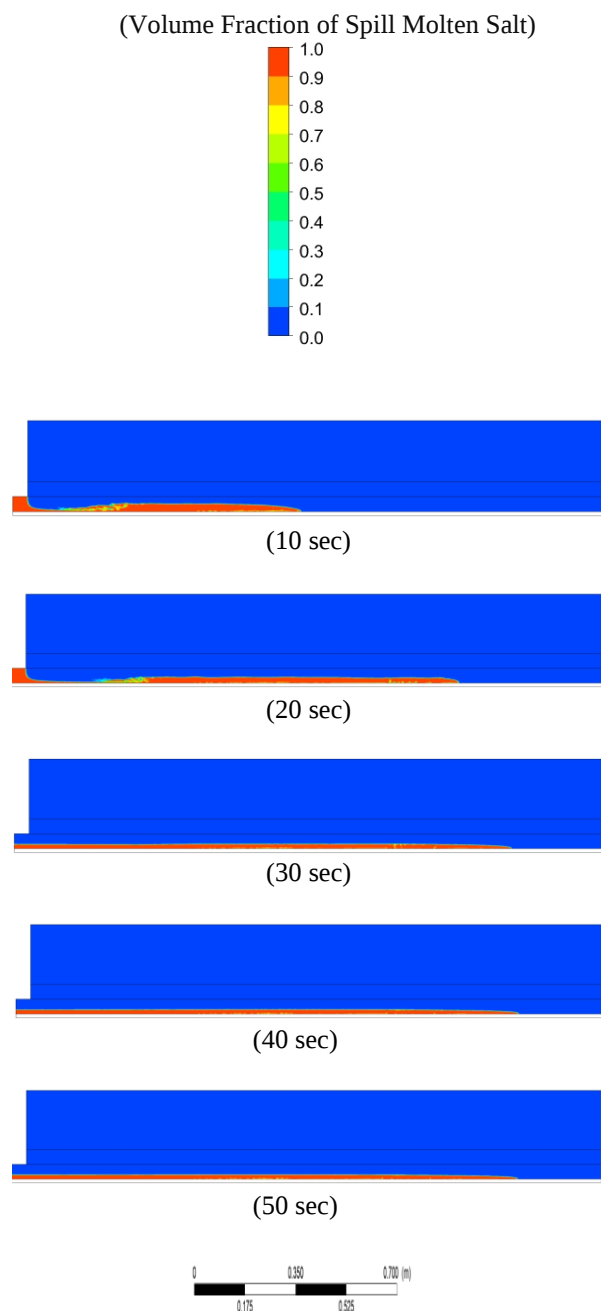
Fig. 3 ANSYS-Fluent results on spreading distance of the spill molten salt with time increase (KCl-NaCl- \text{UCl}_3 ).
