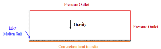
Fig. 1 ANSYS-Fluent input model for spreading analysis of the spill molten salt.
