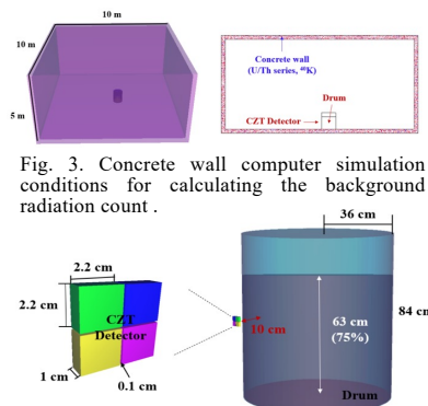
Fig. 4. Conditions for computer simulation of MDA using a CdZnTe detector.
