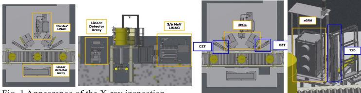
Fig. 1 Appearance of the X-ray inspection equipment proposed by KAERI (left: plan view, right: side view)
