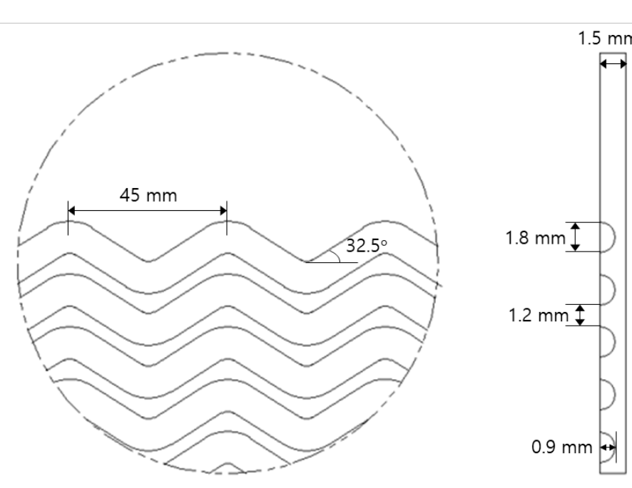
▲ Fig. 3. Detailed channel geometry of PCHE recuperator
