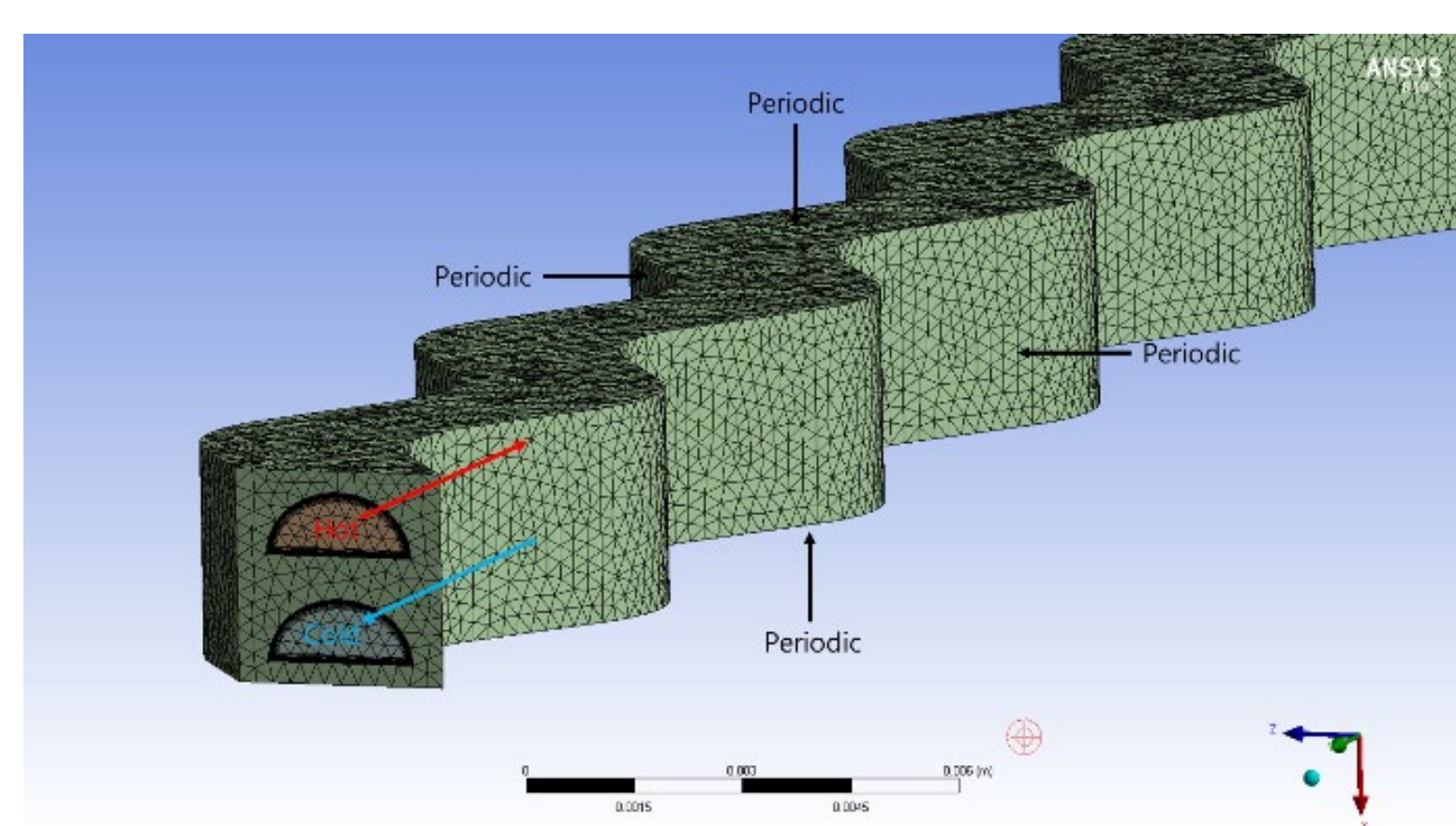
▲ Fig. 4. Computational domain and boundary conditions
