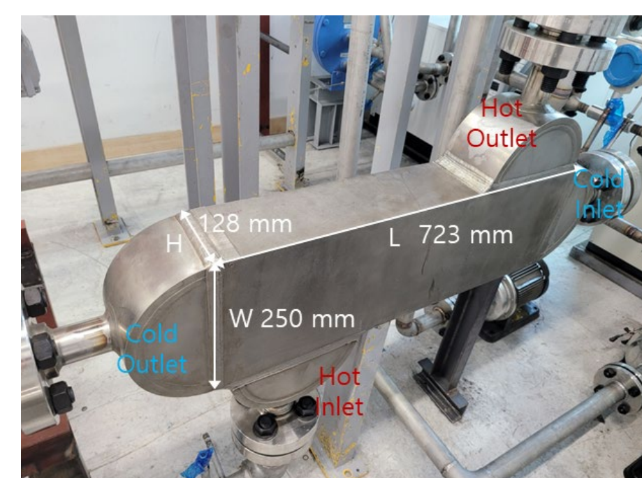
▲ Fig. 2. PCHE recuperator in experimental loop
