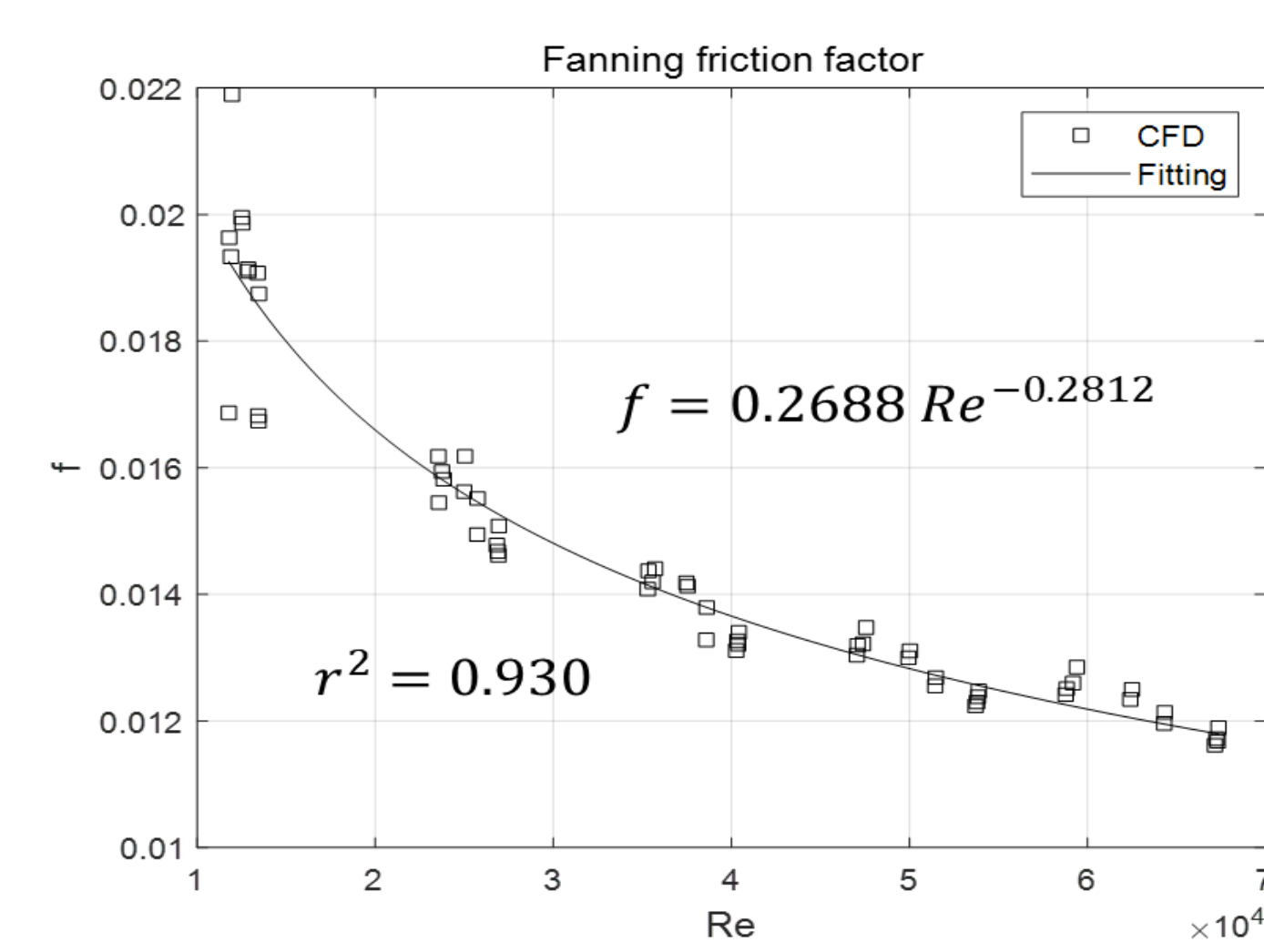
▲ Fig. 6. Result of Fanning friction factor
