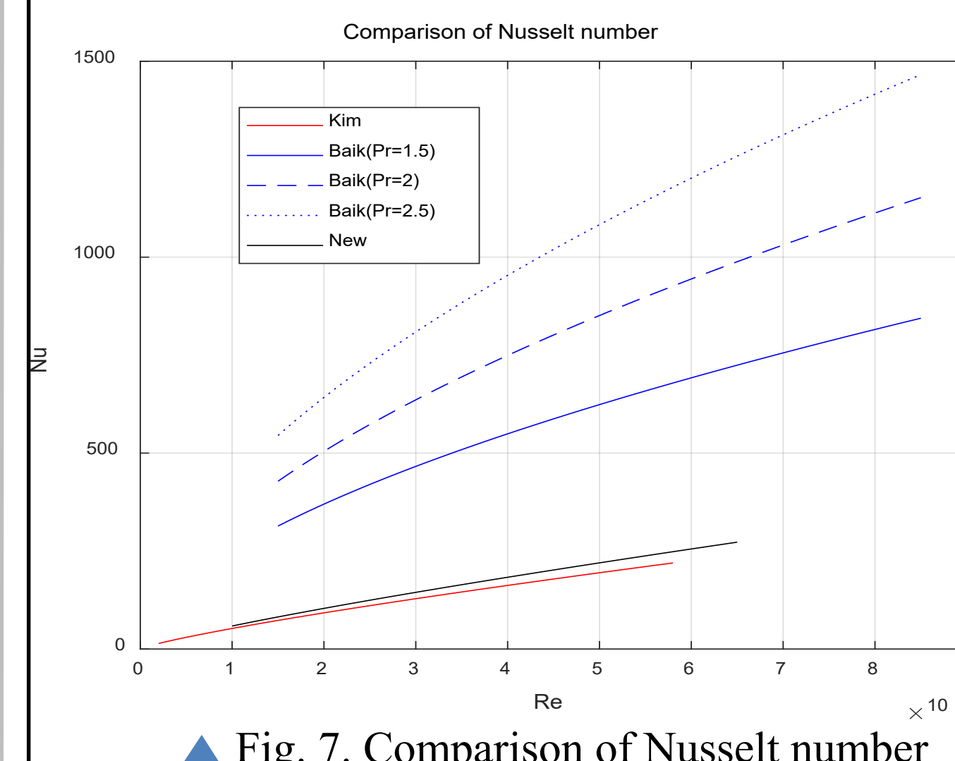
▲ Fig. 7. Comparison of Nusselt number
