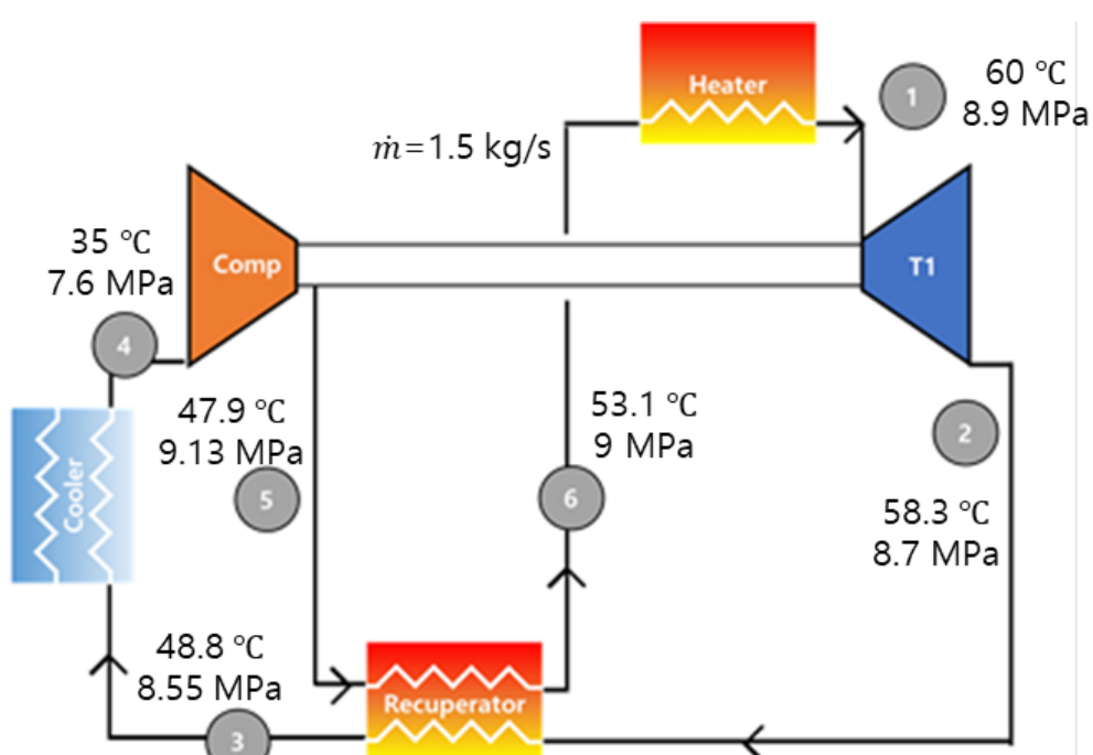
▲ Fig. 1. Schematic diagram of experimental facility and design conditions
