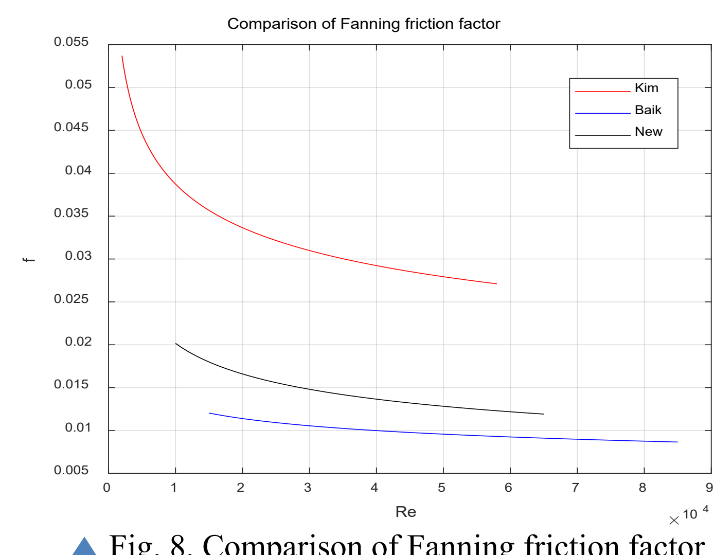
▲ Fig. 8. Comparison of Fanning friction factor
