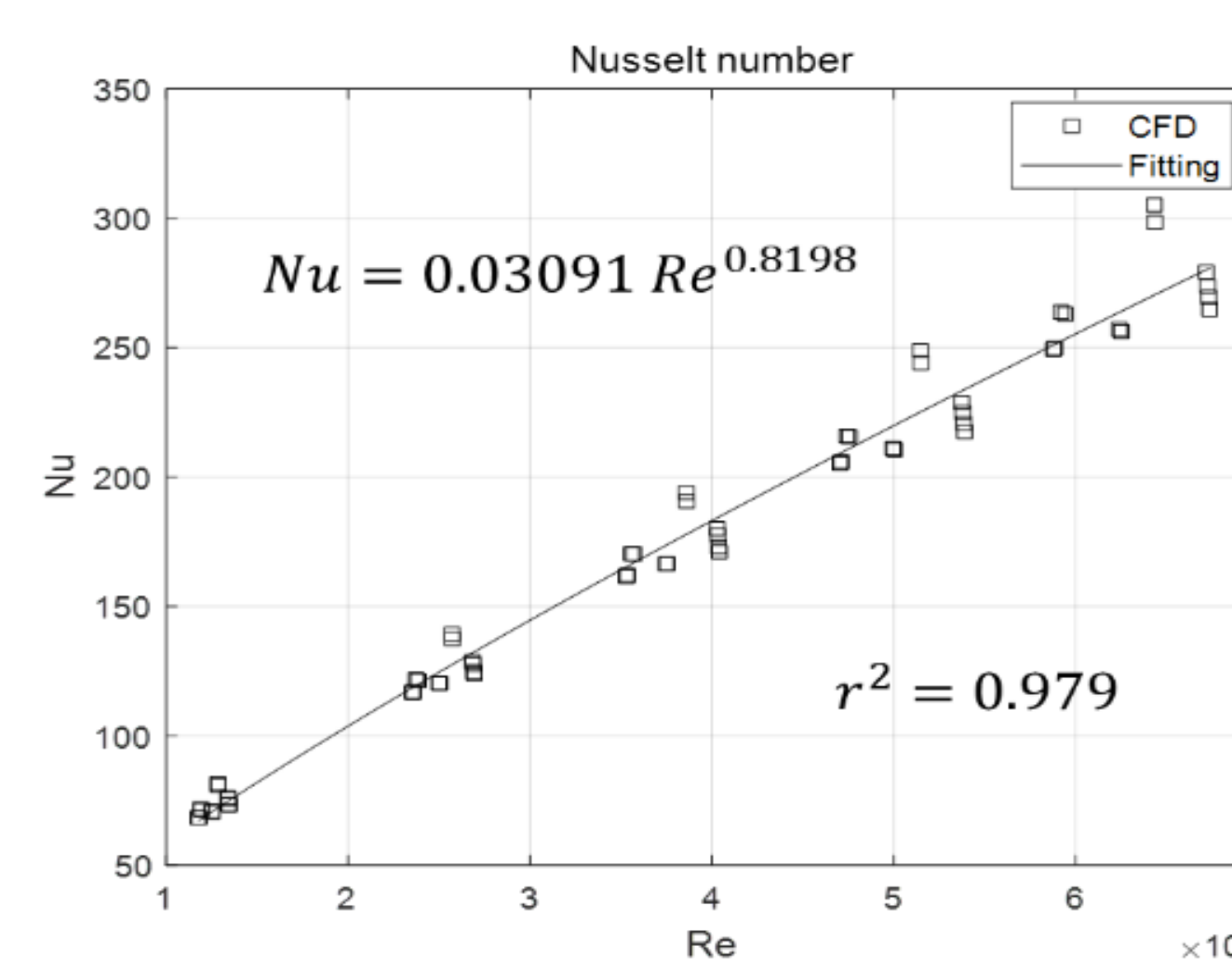
▲ Fig. 5. Result of Nusselt number
