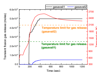
Figure 3. Transient fission gas release with temperature limit for gas release.
