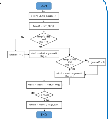
Figure 2. Gas available fraction mapping from FRAPCON to MERCURY
