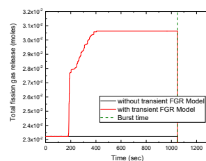
Figure 4. Comparison of total fission gas release with and without transient FGR model.
