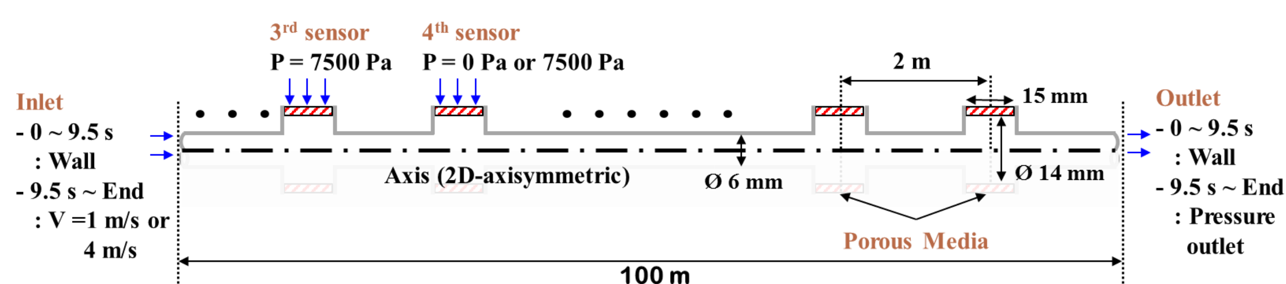
Fig. 1. Analysis domain and boundary conditions for numerical analysis.
