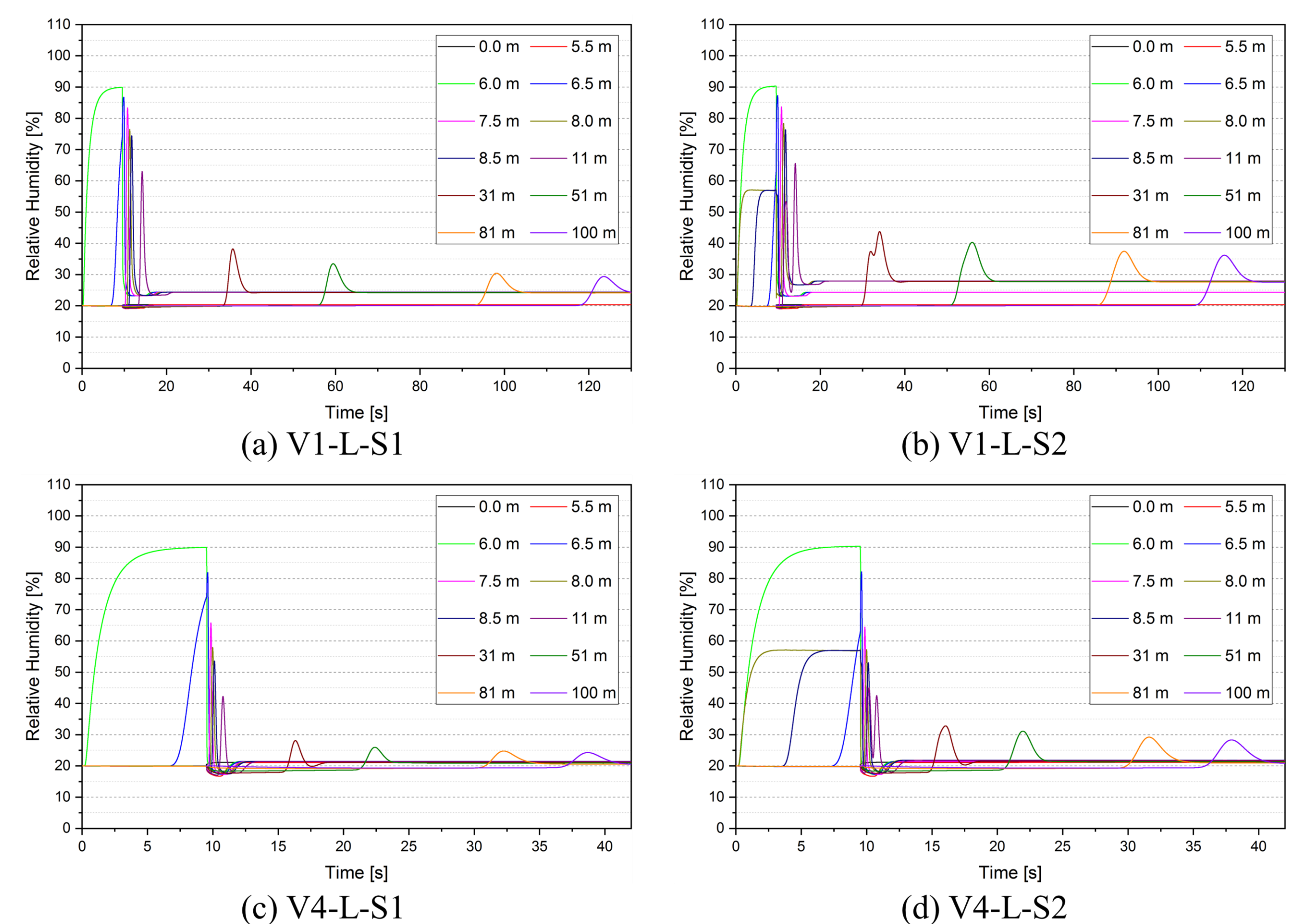
Fig. 2. Relative humidity change in the vertical sections by axial locations.
