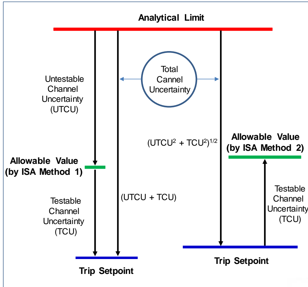
Fig. 1. ISA 67.04 allowable value calculation methods for rising trip parameter
