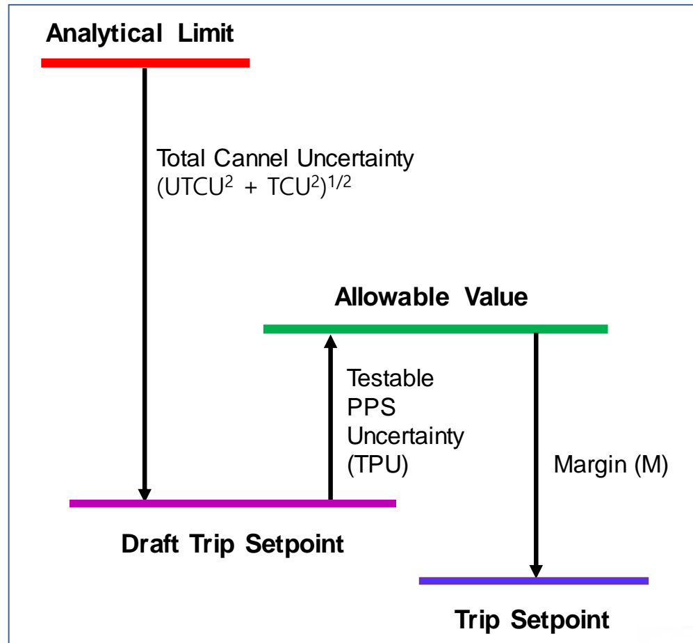
Fig. 2. APR1400 allowable value calculation method for rising trip parameter
