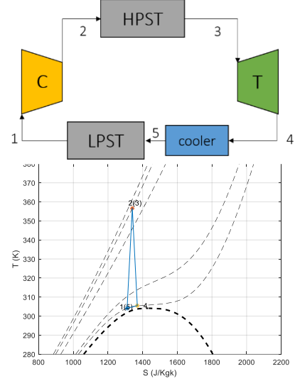
Fig. 2. Simple CCES model with T-S diagram
