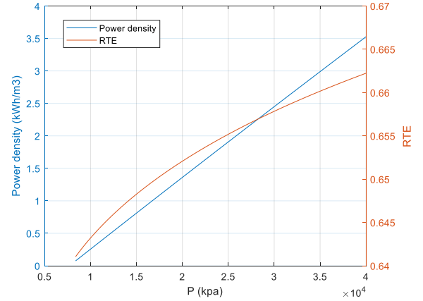
Fig. 3. Sensitivity of a compressor exit pressure - power density and RTE
