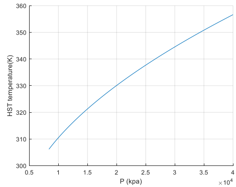
Fig. 9. Temperature change of HPST according to compressor outlet pressure
