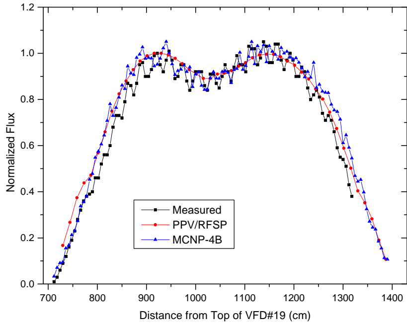
Fig. 1. Vertical Flux Scan for Nominal Case
