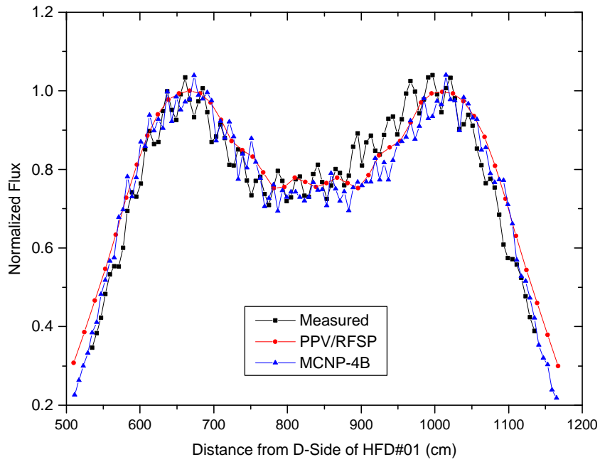
Fig. 2. Horizontal Flux Scan for Nominal Case
