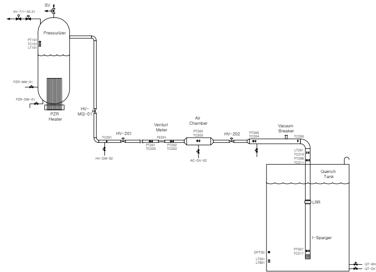
그림 1 Arrangement of Major Components and Instruments of the B&C Loop
