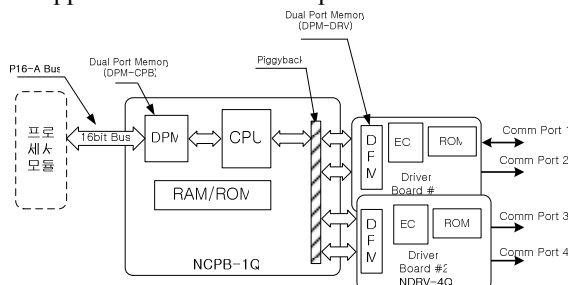
Fig. 1 The H/W Configuration of the HR-SDL Communication Module
