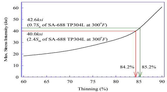
Figure 6. Minimum wall thickness required for the LP heater No. 1 of Ulchin NPP No. 3 & 4 at design condition.
