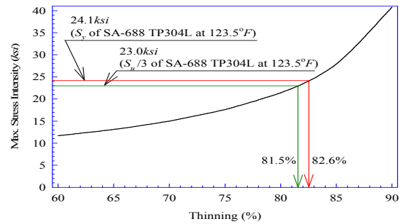
Figure 5. Minimum wall thickness required for the LP heater No. 1 of Ulchin NPP No. 3 & 4 at normal operation.
