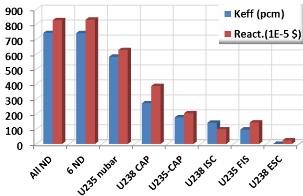
Fig. 3. Uncertainty Decomposition of k-eff and Reactivity Data.
