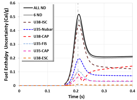
Fig. 9. Time Evolution of Relative Uncertainties in Maximum Nodal Fuel Enthalpy.
