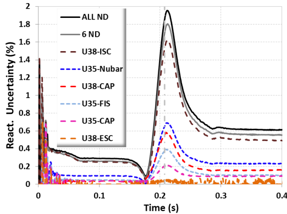
Fig. 7. Time Evolution of Relative Uncertainties in Reactivity
