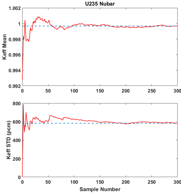
Fig. 2. k-eff Mean and STD Convergence-U-235 Nubar.
