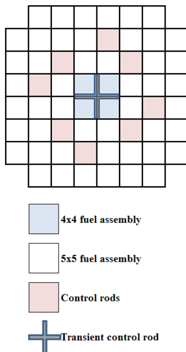
Fig. 1. Layout of the SPERT-III E-core.
