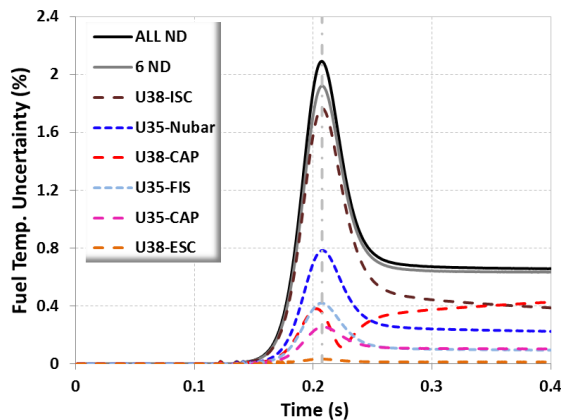
Fig. 8. Time Evolution of Relative Uncertainties in Maximum Nodal Fuel Temperature.
