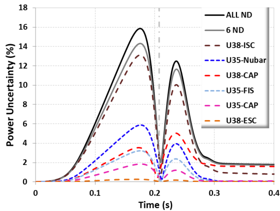
Fig. 6. Time Evolution of Relative Uncertainties in Power.
