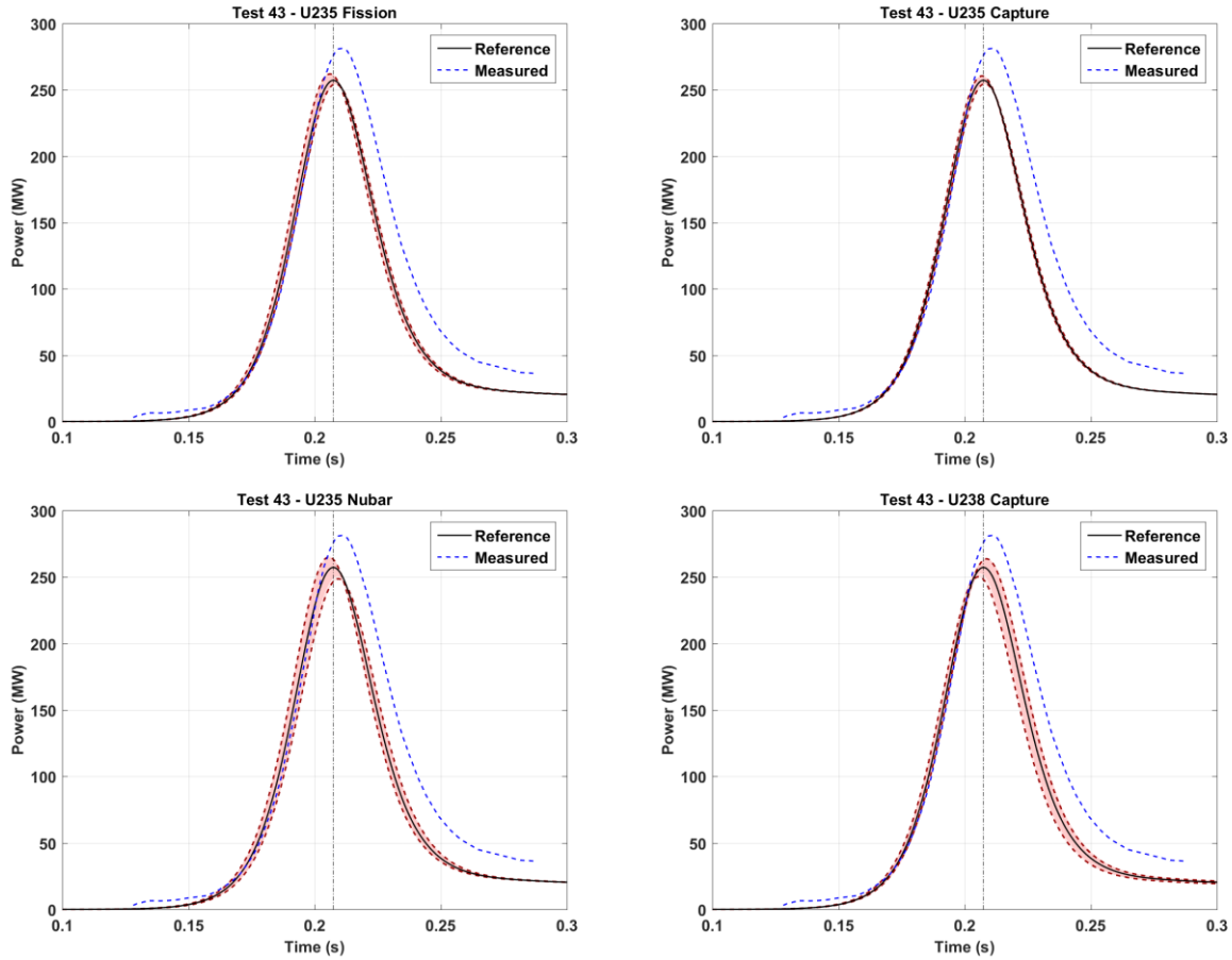
Fig. 5. Time Evolution of Total Power for cases with perturbation of: U-235 Fission (Top-left), U-235 Capture (Top-right), U-235 Nubar (Bottom-left), and U-238 Capture (Bottom-right).
