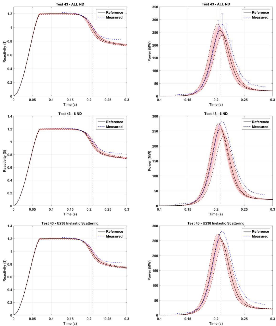
Fig. 4. Time Evolution of Reactivity and Total Power for cases with perturbation of: All ND (Top), 6 ND (Middle), Dominant ND, U-238 Inelastic Scattering (Bottom).
