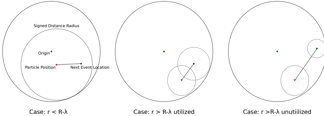
Fig. 9: Depiction of modeling cases.
