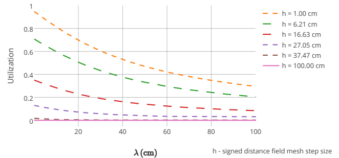
Fig. 11: Results of the model for the theoretical utilization limit with the results of the simulation for a fixed distance traveled case.
