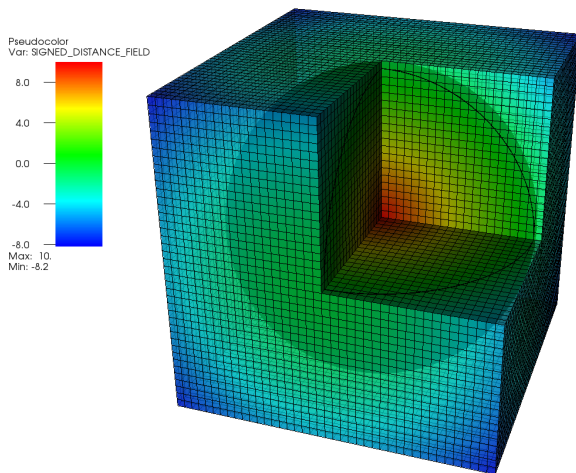
Fig. 3: A visual of a signed distance field with step size 0.5 cm surrounding a spherical test case with radius 10 cm.
