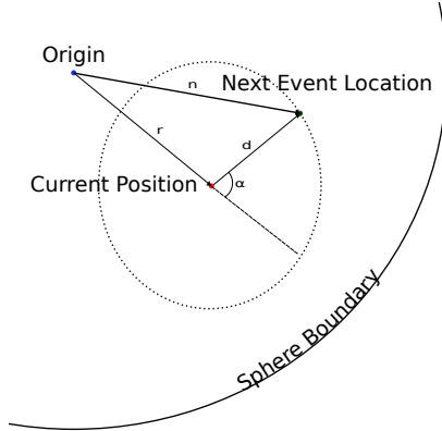
Fig. 8: Depiction of model variables.
