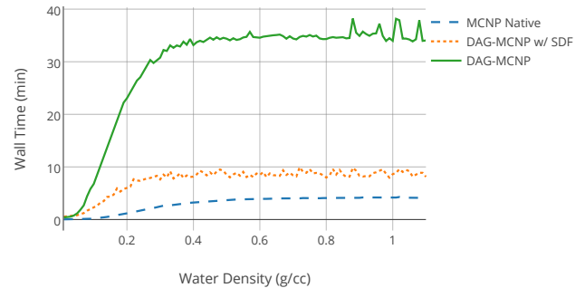
Fig. 5: Performance results for a 5 MeV neutron source at the origin of a 10 cm radius sphere. Water density was varied from 0 to 1 \frac{g}{cm^3} . Simulations of 100M histories at each density were performed using native MCNP5, DAG-MCNP5 without the signed distance field, and DAG-MCNP5 with the signed distance field.
