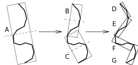
Fig. 1: 2D example of a Bounding Volume Hierarchy using Oriented Bounding Boxes on a discretized curve.
