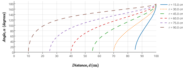
Fig. 10: Plot of minimum angle of departure restriction for particles with various radial positions in a sphere with R = 100 cm and varying distances traveled.
